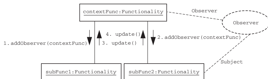
FIGURE 8.20 Using the Event pattern for combination tools.
