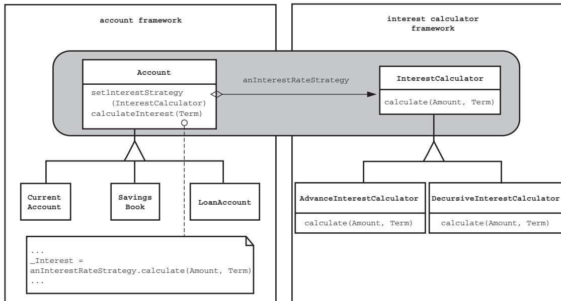
FIGURE 4.3 Example showing an interest rate calculator.
