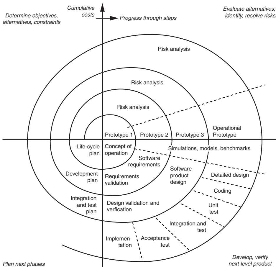
FIGURE 12.3 Example of a spiral model
