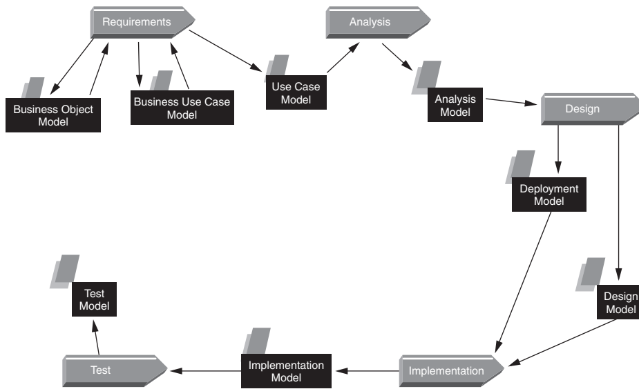
FIGURE 12.22 Up models and workflows.
