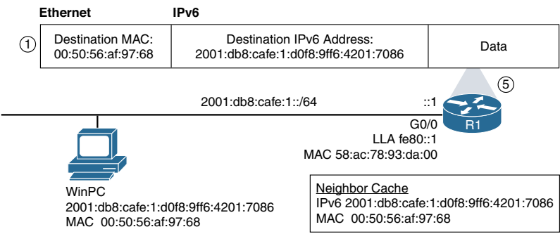
Figure 13-10 R1 Updates Its Neighbor Cache and Forwards the Frame
