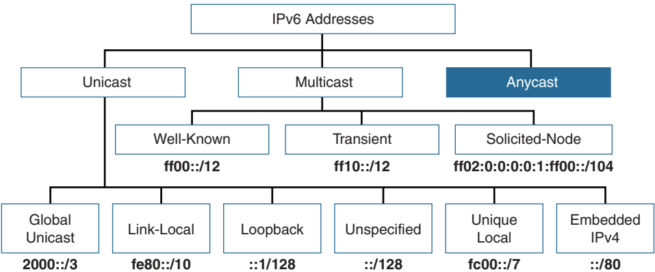
Figure 4-13 Anycast Addresses
