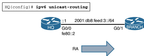
Figure 14-2 Topology for NDp and ND
