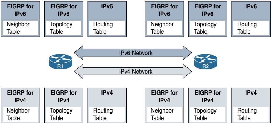
Figure 15-1 Separate EIGRP Tables and Routing Tables for IPv4 and IPv6
