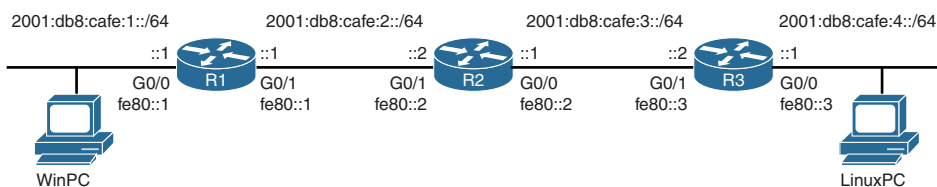
Figure 17-9 IPv6 Topology for ACLs
