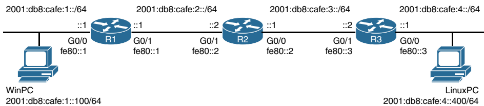
Figure 6-11 Topology Used to Verify Link-Local Addresses
