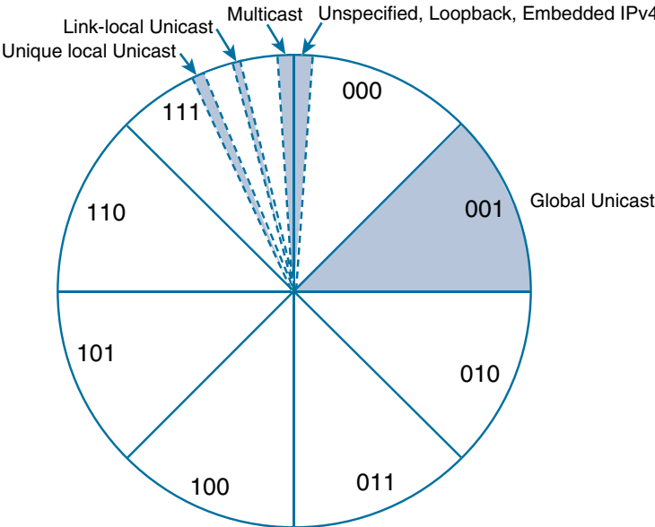
Figure 4-5 IANA's Allocation of IPv6 Address Space in 1/8 Sections
