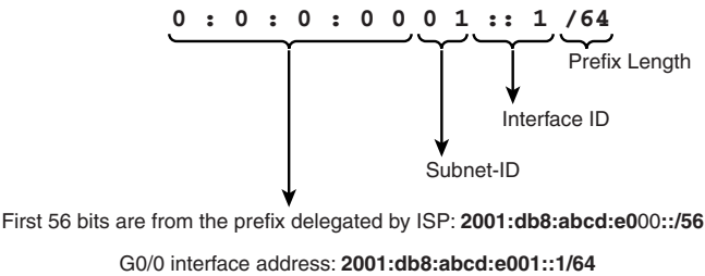
Figure 11-7 ipv6 address General Prefix Command
