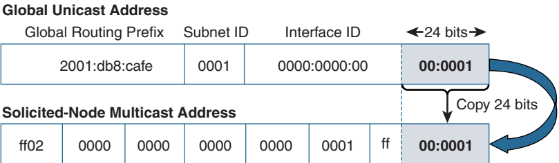
Figure 7-7 Mapping R1's Global Unicast Address to a Solicited-Node Multicast Address
