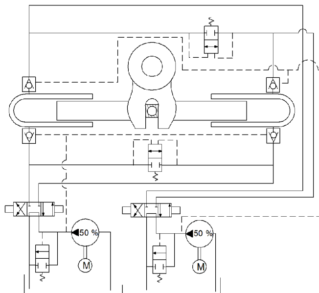
Figure 10 “Appendix A” (see DNV-RU-SHIP Pt.4 Ch.10 App.A) steering gear – two ram type
