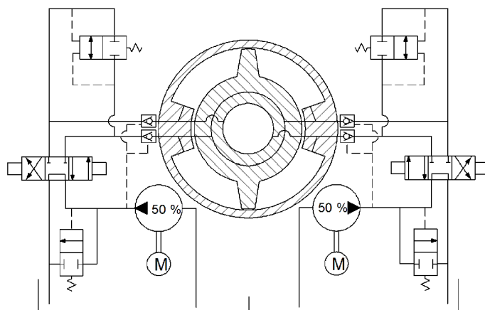
Figure 11 “Appendix A” (see DNV-RU-SHIP Pt.4 Ch.10 App.A) steering gear – rotary vane type
