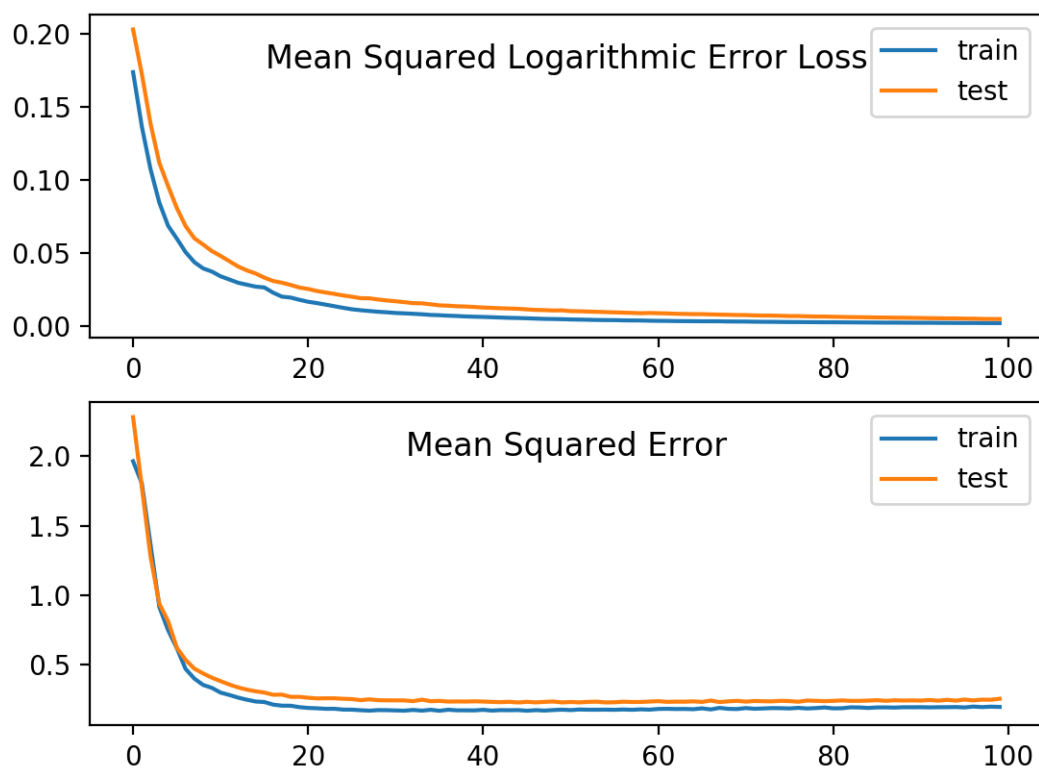
Figure 4.2: Line Plots of Mean Squared Logistic Error Loss and Mean Squared Error Over Training Epochs.
